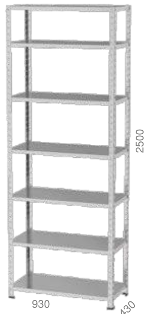
> 25943 930 X 430 X 2500 mm
